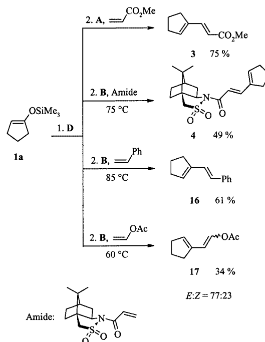
Scheme 5. A: Pd(OAc) 2 , n Bu 4 NCl, K 2 CO 3 , DMF, room temp., 6 h; B: Pd(OAc) 2 , KOAc, K 2 CO 3 , DMF, 6 h; D: n Bu 4 NF, NfF, THF, room temp., 16 h
