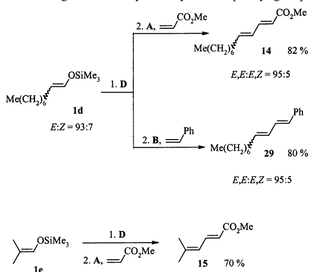
Scheme 9. A : Pd(OAc) 2 , nBu 4 NCl, K 2 CO 3 , DMF, room temp., 6 h; B : Pd(OAc) 2 , KOAc, K 2 CO 3 , DMF, 75 °C, 6 h; D : nBu 4 NF, NfF, THF, room temp., 16 h
