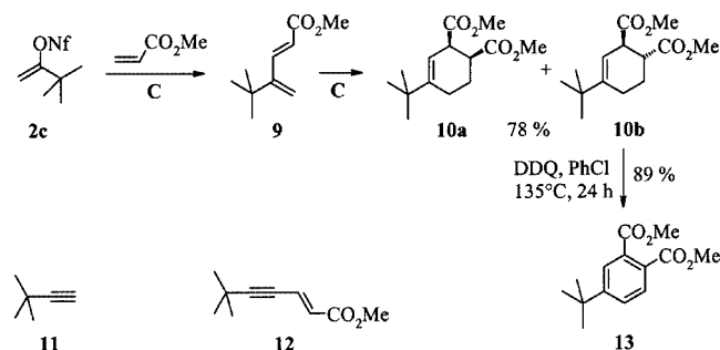
Scheme 3. C : \text{Pd}(\text{OAc})_2 , LiCl, \text{Et}_3\text{N} , THF, 58 °C, 60 h
