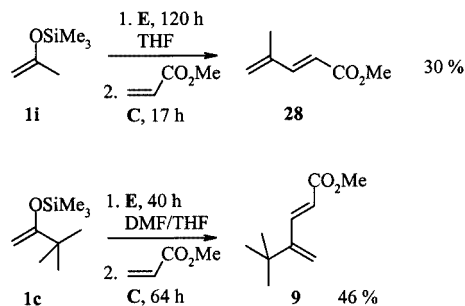
Scheme 8. C : \text{Pd}(\text{OAc})_2 , LiCl, \text{Et}_3\text{N} , DMF/THF, room temp.; E : dibenzo-18-crown-6, KF, NfF, room temp.
