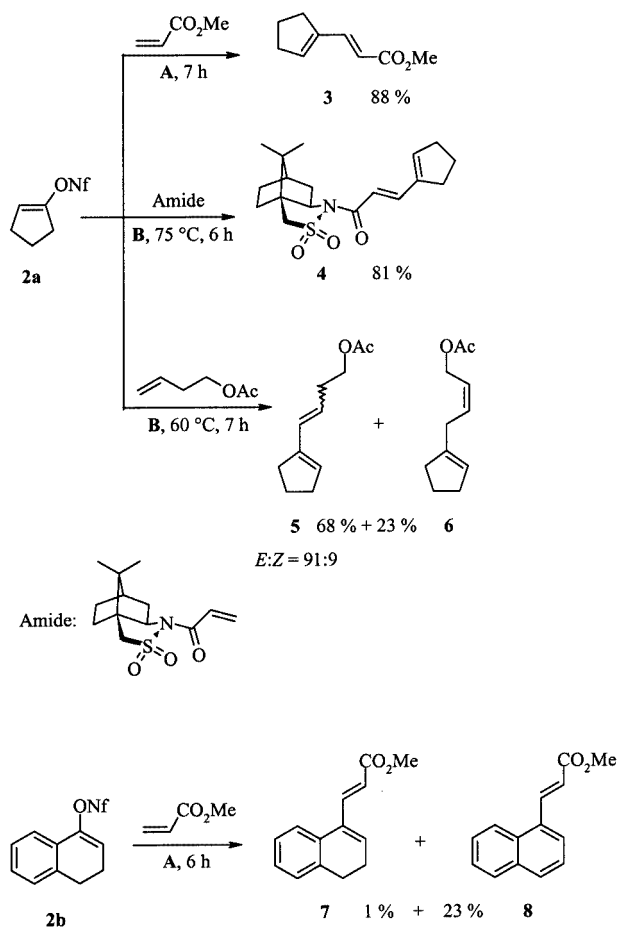
Scheme 2. A : \text{Pd}(\text{OAc})_2 , n\text{Bu}_4\text{NCl} , \text{K}_2\text{CO}_3 , DMF, room temp.; B : \text{Pd}(\text{OAc})_2 , KOAc, \text{K}_2\text{CO}_3 , DMF
