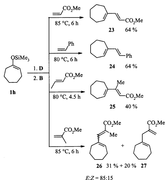
Scheme 7. B : \text{Pd}(\text{OAc})_2 , KOAc, \text{K}_2\text{CO}_3 , DMF; D : n\text{Bu}_4\text{NF} , NfF, THF, room temp., 16 h
